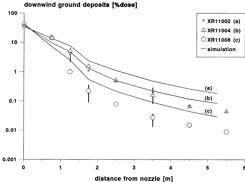
Fig. 5. Downwind spray deposits using different nozzle types. Other parameter settings equal the reference situation. Symbols refer to experimental data. Solid lines with indices (a–c) refer to simulations. Error bars indicate typical deviations between lowest and highest value, for finest and coarsest nozzle.
