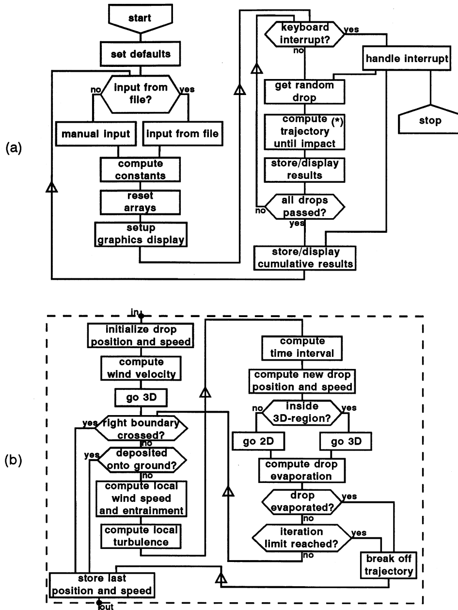
Fig. 2. Flow scheme of the IDEFICS drift model (a). The actual trajectory computations take place in the block marked with an asterisk (*). The structure of this block is shown in detail in (b).
