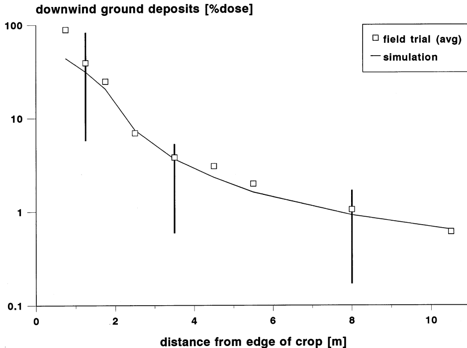
Fig. 9. Comparison of downwind spray deposits in practical field trial (average of four replications) and simulation results. Sprayed volume, 300 l/ha; wind velocity, 3.5 m/s; and boom height, 0.7 m above mature potato crop. Error bars indicate typical deviations between lowest and highest value.
