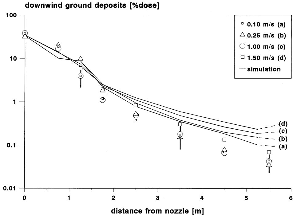
Fig. 7. Downwind spray deposits at various driving speeds. Other parameter settings equal the reference situation. Symbols refer to experimental data. Solid lines with indices (a–d) refer to simulations. Error bars indicate typical deviations between lowest and highest value, for driving speed 1.0 m/s.
