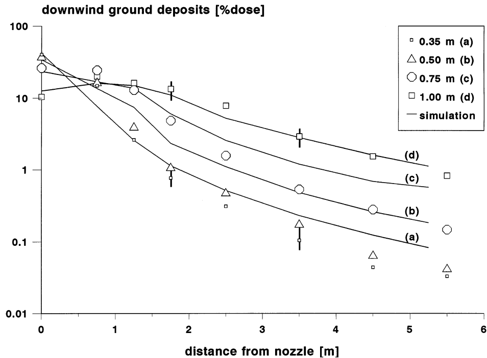
Fig. 4. Downwind spray deposits at various boom heights. Other parameter settings equal the reference situation. Symbols refer to experimental data. Solid lines with indices (a–d) refer to simulations. Error bars indicate typical deviations between lowest and highest value, for lowest and highest boom.
