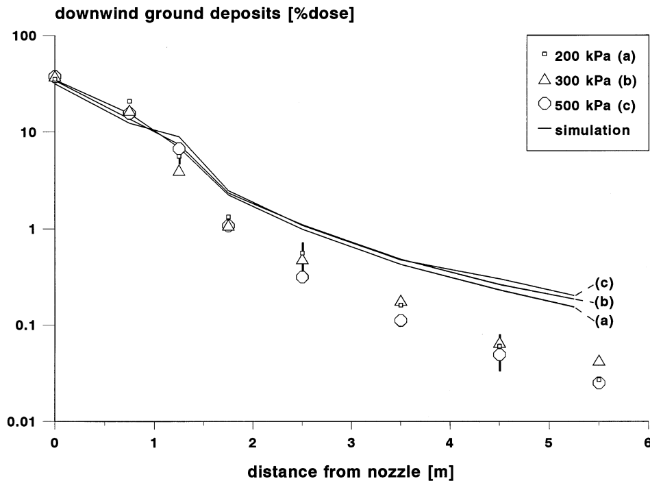
Fig. 6. Downwind spray deposits at different liquid pressures. Other parameter settings equal the reference situation. Symbols refer to experimental data. Solid lines with indices (a–c) refer to simulations. Error bars indicate typical deviations between lowest and highest value, for lowest pressure.
