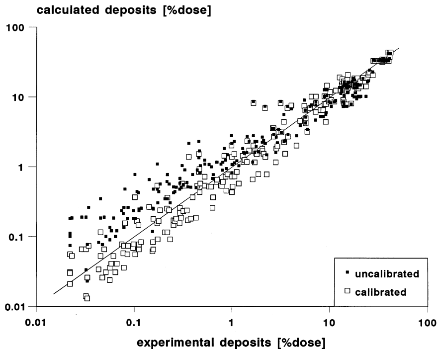
Fig. 8. Correlation between measured and calculated deposits, before and after calibration. The solid line shows the ideal relationship ( y = x ).
