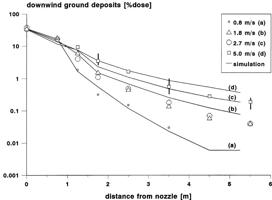
Fig. 3. Downwind spray deposits at various averaged wind velocities. Other parameter settings equal the reference situation. Symbols refer to experimental data. Solid lines with indices (a–d) refer to simulations. Error bars indicate typical deviations between lowest and highest value.
